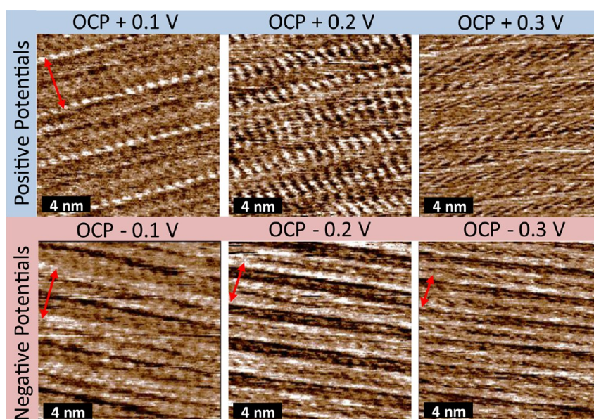
Figure 7. AM-AFM phase images of the EMIm TFSI + 0.1 wt/wt % EMIm Cl Stern layer adsorbed to a graphite (HOPG) substrate. Image sizes are all 15 nm \times 15 nm. The interfacial data were collected at differing applied potentials (indicated in the figure). The slow scan direction of all images is down the image. The red arrow indicates the larger repeat spacing of the image.
