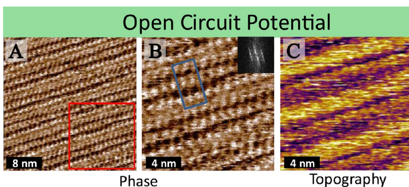
Figure 6. AM-AFM phase (mocha) and topographic (orange–violet–yellow) images of the EMIm TFSI + 0.1 wt/wt % EMIm Cl Stern layer adsorbed to a graphite (HOPG) substrate. The interfacial data were collected at OCP (0.42 V vs Pt). The slow scan direction of all images is down the image. The FFT of the phase image is shown as an inset. The area in the red box in (A) is expanded in (B,C). The blue box indicates the unit cell of the surface ions.
