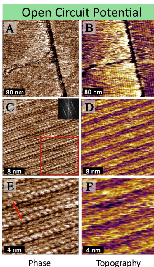
Figure 2. AM-AFM phase (mocha) and topographic (orange–violet–yellow) images of the IL Stern layer adsorbed to a graphite (HOPG) substrate. Image sizes are (A,B) 300 \text{ nm} \times 300 \text{ nm} , (C,D) 30 \text{ nm} \times 30 \text{ nm} , and (E,F) 15 \text{ nm} \times 15 \text{ nm} . The interfacial images were collected at OCP ( 0.26 \text{ V vs Pt} ). The slow scan direction of all images is down the image. The fast Fourier transform of the phase image is shown as an inset. The red arrow indicates the larger repeat spacing of the image. The area in the red box in (C) is expanded in (E,F).
