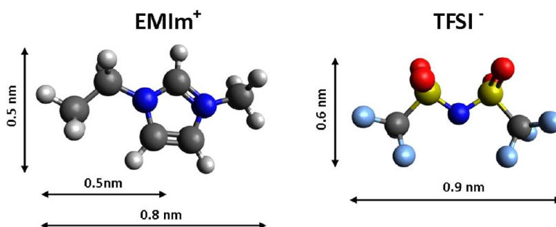
Figure 1. Structure and dimensions of EMIm TFSI. Carbon atoms are shaded gray, nitrogen is dark blue, hydrogen is silver, oxygen is red, sulfur is yellow, and fluorine is light blue.
