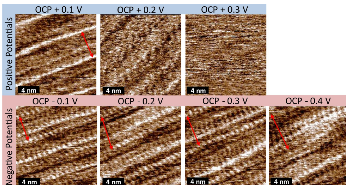
Figure 5. AM-AFM phase (mocha) images of the EMIm TFSI + 0.1 wt/wt % Li TFSI Stern layer adsorbed to a graphite (HOPG) substrate. Image sizes are all 15 \text{ nm} \times 15 \text{ nm} . The interfacial data were collected at differing applied potentials (indicated in the figure). The slow scan direction of all images is down the image. The red arrow indicates the larger repeat spacing of the image.
