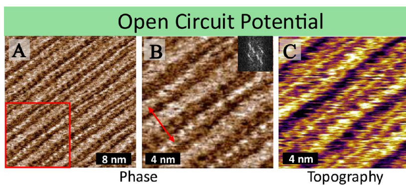
Figure 4. AM-AFM phase (mocha) and topographic (orange–violet–orange) images of the EMIm TFSI + 0.1 wt/wt % Li TFSI Stern layer adsorbed to a graphite (HOPG) substrate. The interfacial data were collected at OCP (0.31 V vs Pt). The slow scan direction of all images is down the image. The FFT of the phase image is shown as an inset. The area in the red box in (A) is expanded in (B,C).
